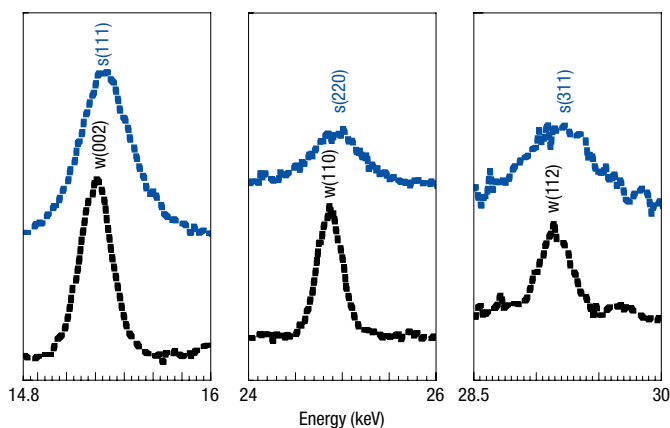
Figure 4 Comparison of the three characteristic X-ray-diffraction peaks between wurtzite and sphalerite polymorphs at 1 atm pressure. Here w and s represent the wurtzite and sphalerite, respectively.
