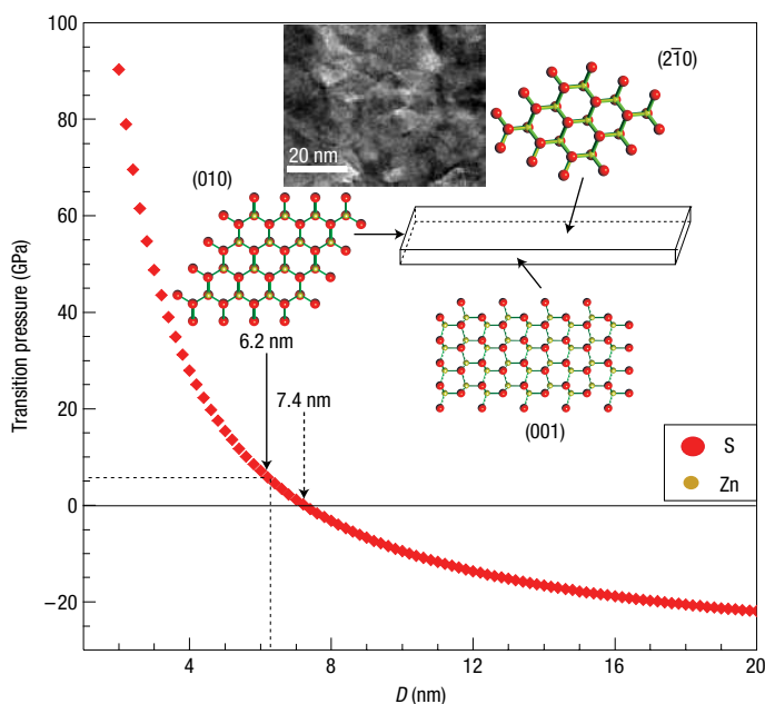
Figure 3 Correlation between the nano-thickness ( D ) and transition pressure of one-dimensional wurtzite nanobelts. Inset figures show the three characteristic surfaces and the corresponding atomic arrangements in reciprocal lattice demonstrations. Inset HRTEM figure shows that the recovered samples have the cubic and tetragonal shapes with an average size of 10 nm.
