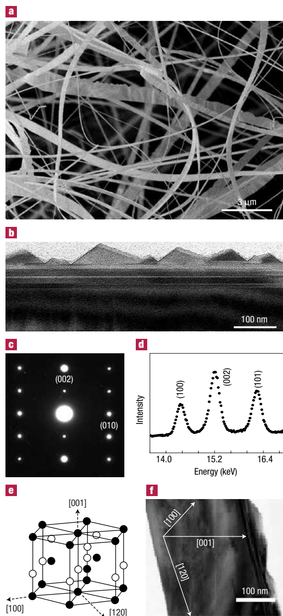
Figure 1 The synthesized wurtzite-structure ZnS nanobelts. a , Low-resolution SEM image; b , HRTEM image showing saw-like edge; c , electron-diffraction image; d , X-ray-diffraction pattern; e , schematic representation of the wurtzite structure; and f , the crystallographic dimensions of nanobelts.
