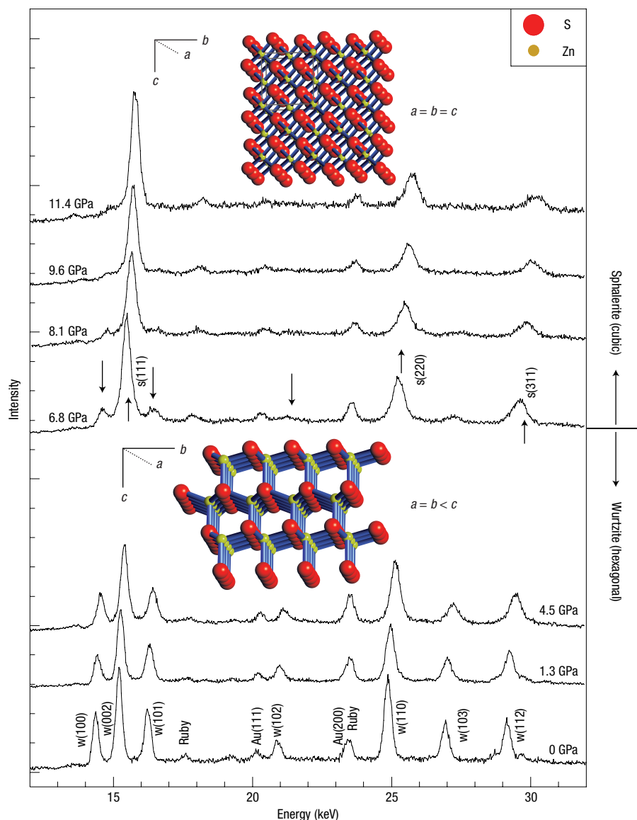
Figure 2 High-pressure X-ray-diffraction patterns of the wurtzite ZnS nanobelts. The upward and downward arrows ( \uparrow and \downarrow ) represent the occurrence and disappearance of X-ray-diffraction peaks of the new cubic phase and hexagonal phase. Their crystallographic characteristics are schematically shown in the two inset figures: bottom for hexagonal wurtzite and top for cubic sphalerite. Weaker X-ray-diffraction peaks are due to the small amount of gold nanoparticles used as a catalyst during synthesis and by the ruby used as a pressure calibrant.
