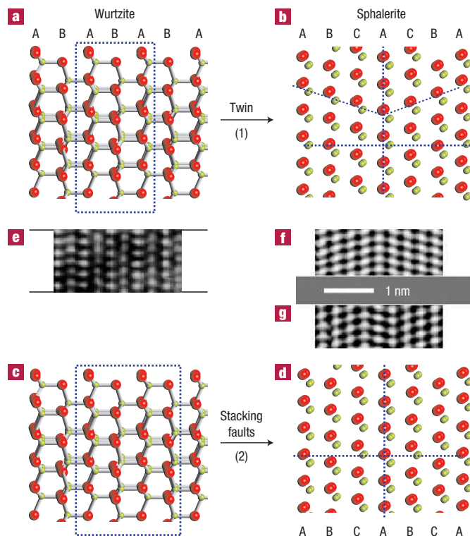
Figure 5 Schematic representation of the wurtzite-to-sphalerite phase transformation. a, b , The first (1) involves the rearrangement of three {ZnS} layers (a), leading to (111) twinning in sphalerite related by a 180^\circ rotation (b). c, d , The second (2) involves the rearrangement of four {ZnS} layers (c), resulting in the development of stacking faults (d). e–g , Filtered HRTEM images of the samples: starting wurtzite phase (e); recovered sphalerite phase (f,g).
