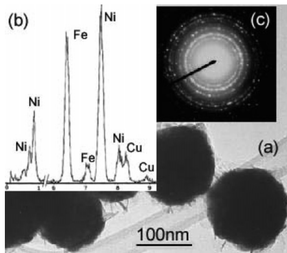
Figure 3. (a) HFTEM image of FeNi 3 alloy; (b) EDS pattern from the FeNi 3 alloy, showing the presence of Fe and Ni in the structure; (c) SAED spectroscopy of FeNi 3 alloy.
