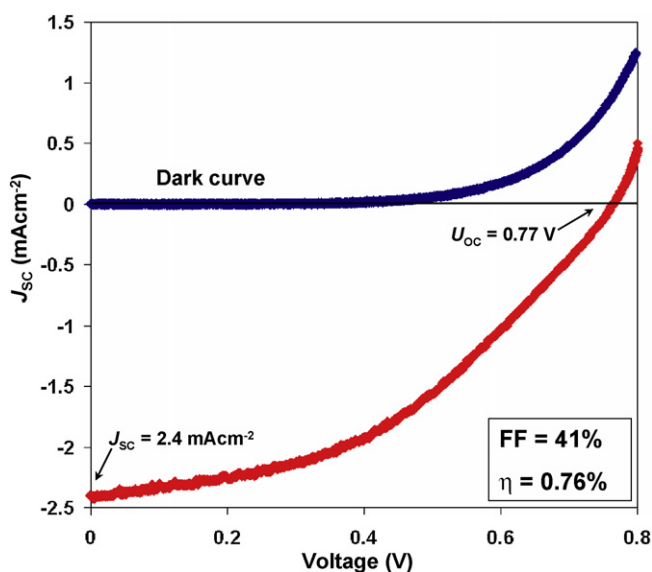
Fig. 31. J - V curve recorded from a DSSC under simulated sunlight. The blue curve is the I - V curve when there is no sunlight illumination, which is a good calibration about the response of the SC. By illuminating with sunlight, the open circuit voltage is 0.77 V and the short circuit current is 240 \mu A and I = 170 \mu A. The fill factor of this DSSC is 41% at the operation point U = 0.471 V and I = 170 \mu A. The energy conversion efficiency was calculated to be 0.76%. From [78]. (For interpretation of the references to color in this figure legend, the reader is referred to the web version of the article.)
