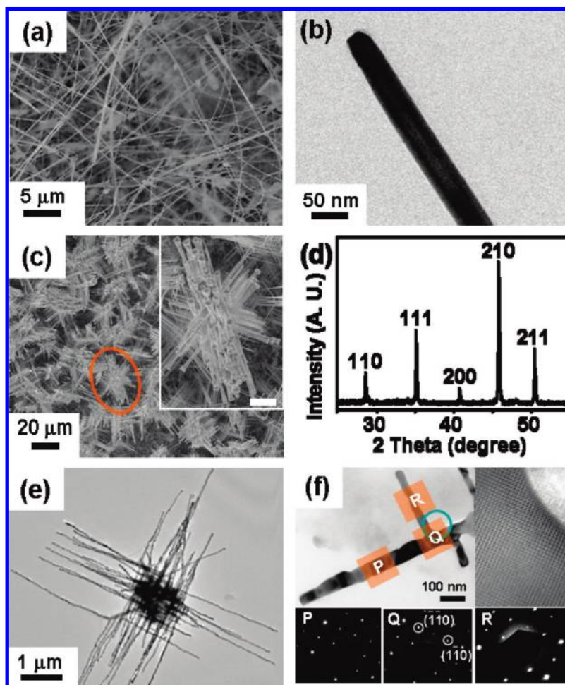
Figure 1. (a) Representative SEM image of CoSi nanowires grown at 750 °C in region A. (b) TEM image of a CoSi nanowire grown at 750 °C in region A. (c) Low-magnification SEM images of the CoSi nanowire networks grown at 780 °C in region A. Inset: High-magnification SEM image. The scale bar is 5 \mu\text{m} . (d) XRD pattern from a sample of CoSi nanowire networks grown at 780 °C in region A. TEM images (e) showing a complete 3D nanowire network and (f) a broken nanowire network segment grown at 780 °C in region A. Insets are the SAEDs from the regions P, Q, and R as well as HRTEM image of an intersection.
