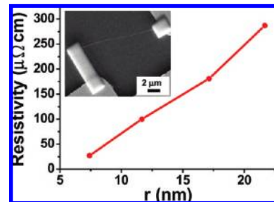
Figure 4. The curve depicting resistivity versus diameter of nanowires. Inset: the SEM image of the measurement structure.
