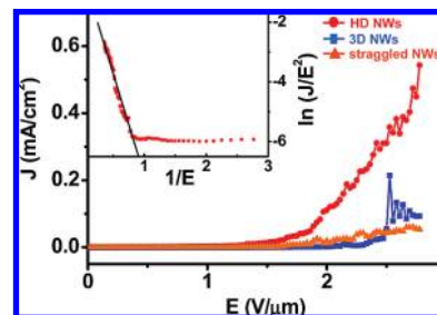
Figure 3. Field emission curves of the three type nanostructures: high density single-stem nanowires (HD NWs), the 3D nanowires networks, and the straggled single-stem nanowires. Inset: the FN plot of high density single-stem nanowires.
