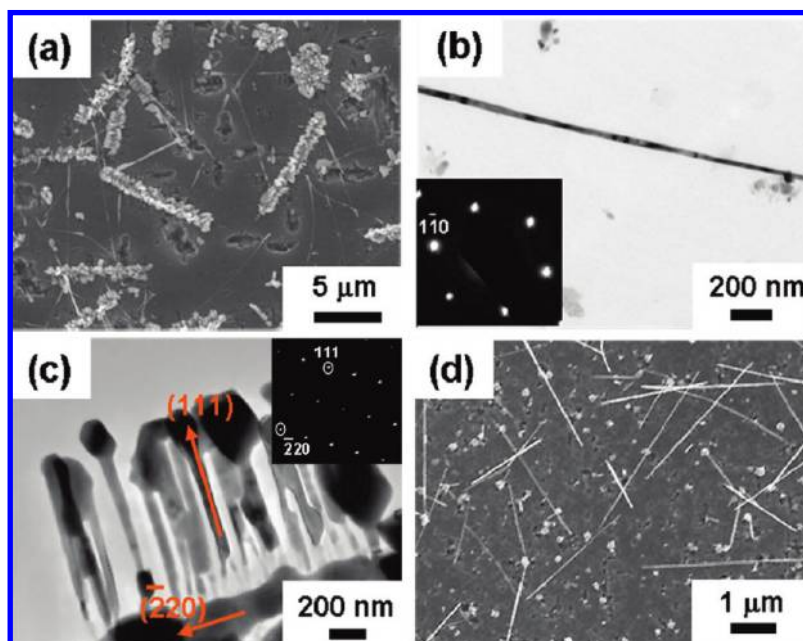
Figure 2. (a) SEM image of \text{Co}_2\text{Si} nanowires formed in region B. TEM images of (b) a single-stem nanowire and (c) aloelike nanostructures. (d) Representative SEM image of straggled \text{CoSi} nanowires grown in region C.
