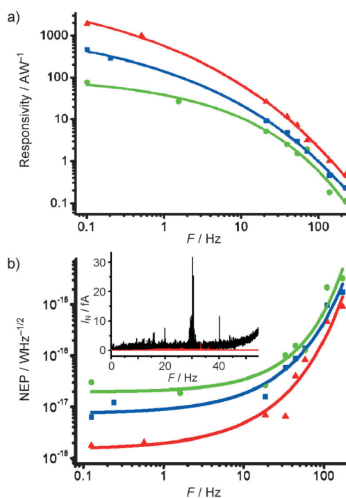
Figure 4. Frequency-dependent performance of the self-powered multicolor NWPD. a) Responsivity versus modulation frequency F under 2.3 \times 10^{-9} \text{W cm}^{-2} UV, blue, and green light illumination. Lines: data fitting. b) Noise-equivalent power (NEP) versus modulation frequency F of the self-powered NWPD for different color light detection. Inset: noise current I_N of the NWPD driven by a hybridized MFC (red) and by a 0.3 V external voltage source (black) provided through a function generator at a bandwidth of 90 Hz (from 10 to 100 Hz).
