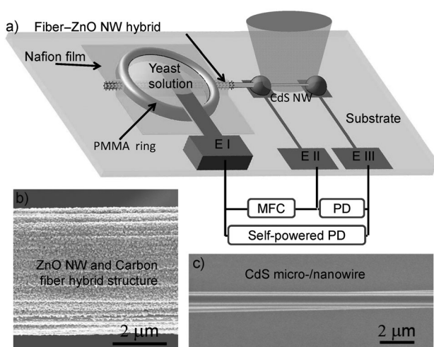
Figure 1. Experimental design of the self-powered photodetector system. a) Illustration of a self-powered nanosystem composed of a microbial fuel cell (MFC) and a nanowire (NW) photodetector (PD). E = electrode. b) SEM image of a carbon fiber covered with densely packed ZnO NWs, which was used for fabricating the MFC. c) SEM image of a CdS wire used for fabricating the photodetector.
