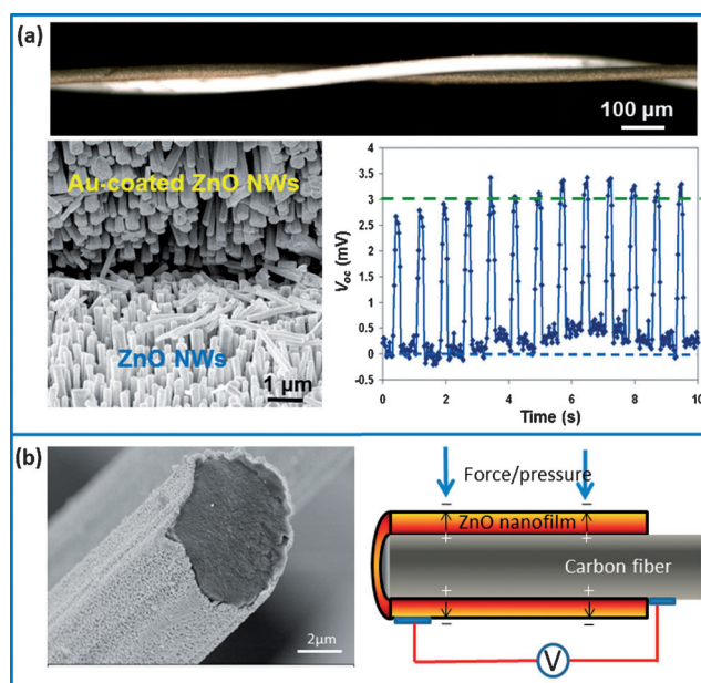
Figure 9. a) Fiber-based nanogenerator based on the principle described in Ref. [95b] (from Ref. [101b]). b) Fiber nanogenerator based on the use of a nanowire film formed on the surface of a carbon fiber (from Ref. [113]). The principle is shown on the right-hand side.
