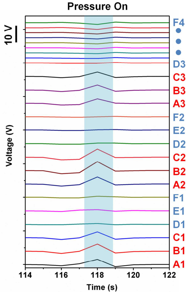
Figure S13. The measured output voltage response of the TEAS matrix with local pressure applied on a quarter of the pixels of the sensor array. The highlighted area in the plot indicates the time period when the pressure is on. The pressure was locally applied on Pixels A1 to C3, which is marked as red in the plot.
