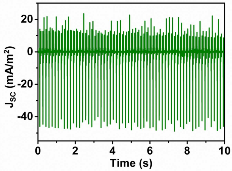
Figure S2. The higher output of the short-circuit current density ( J_{SC} ) with a larger frequency (6 Hz) of the external triggering force. The peak value of the J_{SC} is over 40 mA/m 2 .
