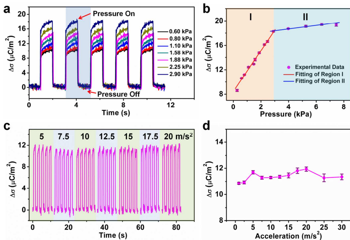
Figure S5. Static pressure sensing by measuring the amount of the transferred charge density ( \Delta\sigma ) upon variable applied pressures. (a) The real-time data \Delta\sigma of the measured with cyclic triggering of the TEAS loaded by variable pressures. The highlighted region shows a full cycle of loading and unloading process, where the pressure “on” and “off” states are pointed out, respectively. (b) The summarized data and linear fittings of the \Delta\sigma with variable applied pressures. Region I is the low pressure region with high sensitivity, while region II is the high pressure region with low sensitivity. The reason for the splitting of the two regions is similar with the case in that of the V_{OC} . (c) The measured \Delta\sigma with a constant pressure (1.2 kPa) but with variable accelerations of the linear motor. (d) The summarized plotting of the measured \Delta\sigma with variable accelerations ranging from 2.5 to 30 \text{m}/\text{s}^2 .
