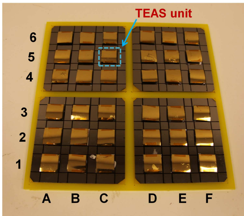
Figure S11. The photograph of the integrated TEAS matrix with a 6×6 array of pressure sensor units. To track the exact position of each pixel, each row was numbered with “1 to 6”, and each column was alphabetically marked with “A to F”.
