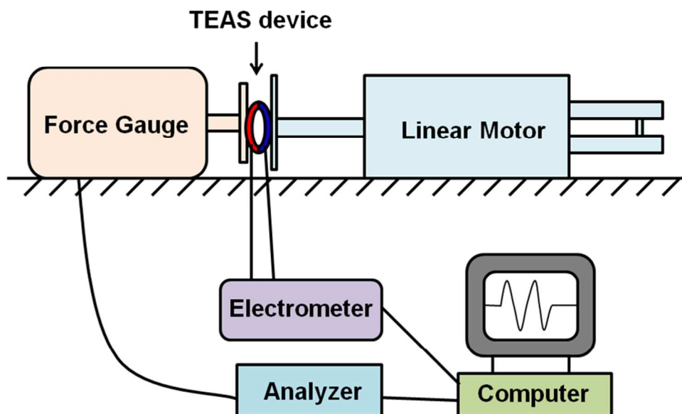
Figure S4. A sketch of the measurement system for characterizing the performance of the TEAS. In this setup, the mechanical linear motor was utilized to apply the external force/pressure onto the TEAS device, and the force gauge was employed for measurement of the real-time force magnitude. Both the data of electrical response and loading force were recorded in the same computer.
