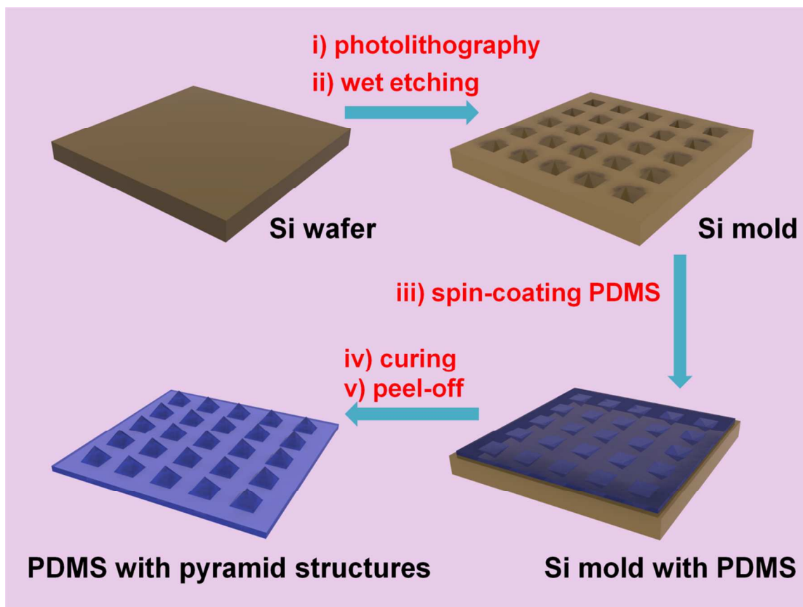
Figure S1. The schematic fabrication process flow of the micro-patterned Polydimethylsiloxane (PDMS) membrane. The (100) Si wafer was used to fabricate the mold for PDMS casting. We first employ the photolithography technique to transfer the patterns from the pre-designed mask to the surface of the Si wafer. Then, the wafer was wet etched with potassium hydroxide solution and the concave pyramid patterns were formed on the Si wafer. In the next step, the mixer of the PDMS elastomer as well as the cross-linker was casted on the surface of the patterned Si mold, and the whole composite was degassed before spin-coating at 500 rpm. Finally, the Si mold with the spin-coated PDMS membrane was placed in a convection oven at 100 °C for two hours when the PDMS got cured, and the PDMS membrane could be peeled off from the Si mold and the pyramid micro-patterned structure was obtained.
