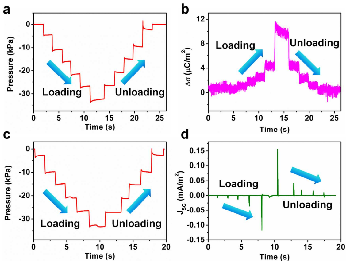
Figure S10. The repeatability test for the pressure-expanded TEAS with step-by-step loading and unloading of the applied pressures. (a) The real-time measurement of the applied pressure with step-by-step loading and unloading in Test 1 for static pressure sensing. (b) The measured \Delta\sigma with a step-by-step behavior corresponding to the pressure recording in (a). (c) The real-time measurement of the applied pressure with step-by-step loading and unloading in Test 2 for dynamic pressure sensing. (d) The measured \Delta\sigma with a multi-pulse behavior corresponding to the pressure recording in (c).
