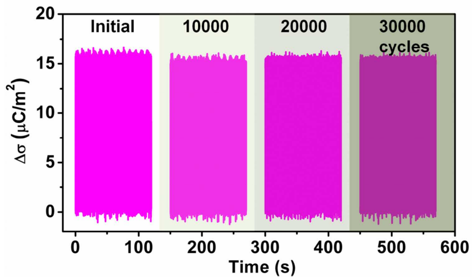
Figure S6. The stability of the measured \Delta\sigma with continuous loading at a constant pressure of 2.5 kPa. The TEAS device was continuously loaded and unloaded with the applied pressure for 30000 cycles, and the data of the \Delta\sigma was measured after every 10000 cycles, and each 300 cycles were recorded and displayed in the plot.
