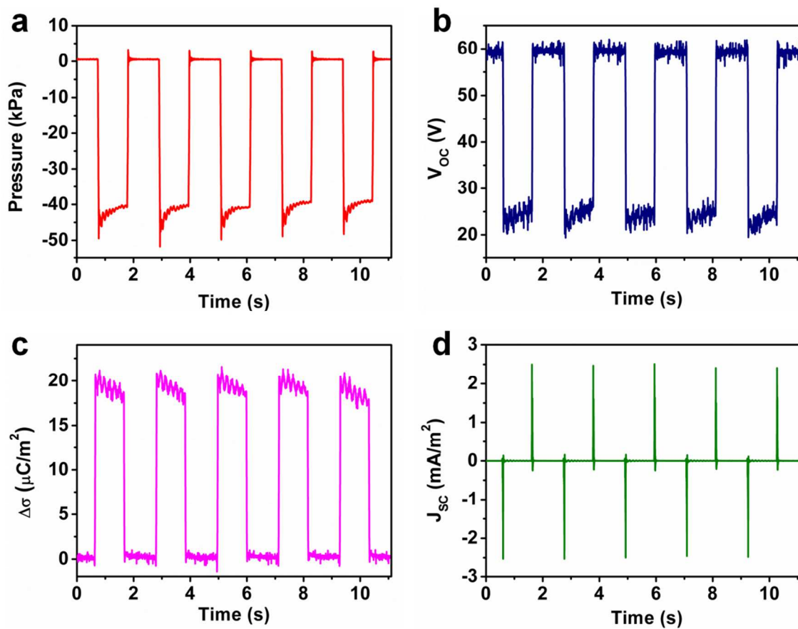
Figure S9. The measured typical electrical response of the pressure-expanded TEAS with a cyclic arbitrary pressure. (a) The real-time measurement of the pressure loaded on the pressure-expanded TEAS device. (b-d) The measured V_{OC} , \Delta\sigma , and J_{SC} corresponding to the applied pressure in (a).
