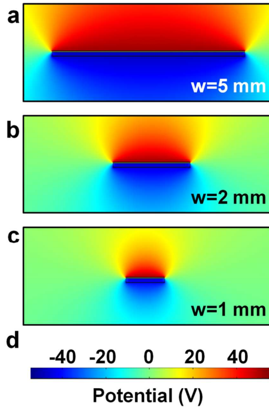
Figure S3. The numerical calculation results for the potential difference between the two electrodes of the triboelectric active sensor (TEAS) with variable device sizes. In the two dimensional model, the difference in device size is represented by the width of the plate ( w ). It can be found that as w varies (5 mm, 2mm, and 1 mm), the potential difference almost remains unchanged ( \sim 90 V). This result demonstrates that the calculation result in Figure 2 could be extended to any size of device with minor variations, and the V_{OC} is a reliable parameter for static pressure sensing.
