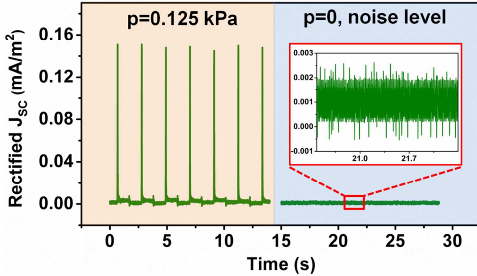
Figure S7. The measurement of the low-end detection limit of the TEAS through the rectified short-circuit current density ( J_{SC} ). The left panel in the plot shows the output J_{SC} with a gentle pressure applied on the TEAS, while the right panel shows the measurement of the noise level magnitude with the same measurement range of the electrometer. The inset is the enlarged view of the J_{SC} for the noise level with no pressure on. With this measurement the low-end detection limit of the TEAS could be deduced with the following equation.
