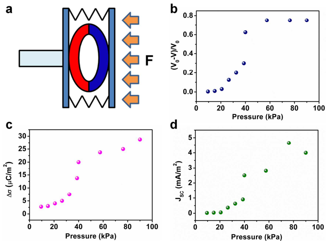
Figure S8. The experimental setup and measurement results for the extension of pressure sensing range. (a) The schematic illustration of the structure and experimental setup for the pressure-expanded TEAS device. (b-d) The measured electrical response of the V_{OC} , \Delta\sigma , and J_{SC} of the pressure-expanded TEAS with variable and higher pressures than those for the tests of the original TEAS device.
