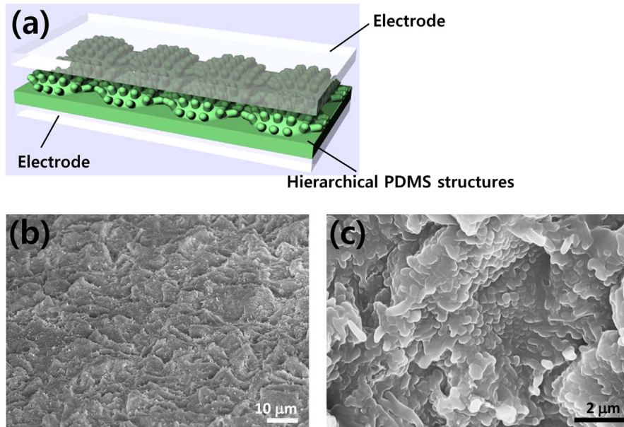
Figure 1 Schematics and SEM images of TENG with hierarchical PDMS structures. (a) Scheme of TENG with PDMS with micro-nano roughness on its surface. (b) SEM image of PDMS surface with micro structure and NWs. (c) Magnified SEM image of PDMS NWs on micro structures.
