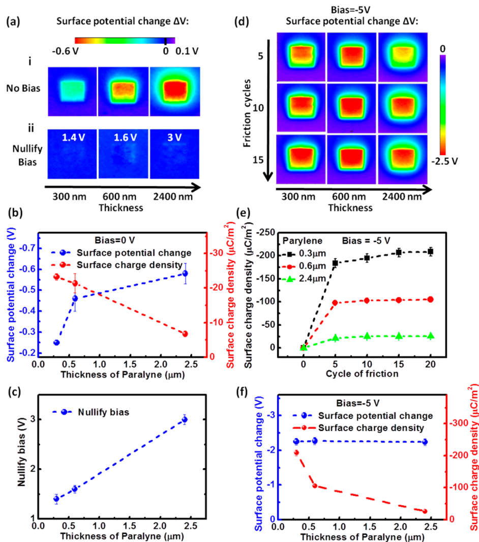
Figure 4. Thickness dependence of contact electrification and bias modulation. (a) Images of surface potential change \Delta V of different thickness samples after they were rubbed at no bias (i) and nullify bias (ii), respectively. (b) The surface potential change and surface charge density as a function of the thickness of the Parylene layer after the sample was rubbed at no bias. (c) The nullify bias as a function of the thickness of the Parylene layer. (d) Images of surface potential change \Delta V of different thickness samples after they were rubbed by different cycles. (e) Calculated surface charge density as a function of friction cycles. (f) The surface potential change and charge density after 20 cycles of friction as a function of thickness of Parylene.
