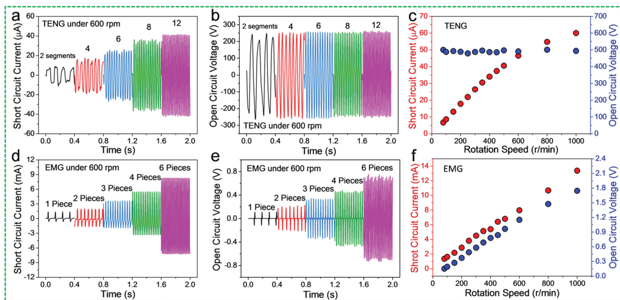
Figure 3. The electrical performance dependence of the TENG and EMG on the parameters. a) The short-circuit current and b) the open-circuit voltage of the TENG with different number of segments. c) The amplitudes of short-circuit current and open-circuit voltage of the TENG with the segmentation of 12 under various rotation speed. d) The short-circuit current and e) the open-circuit voltage of the EMG with different number of coil–magnet pairs. f) The amplitudes of short-circuit current and open-circuit voltage of the EMG with the coil–magnet pairs' number of 6 under various rotation speed.
