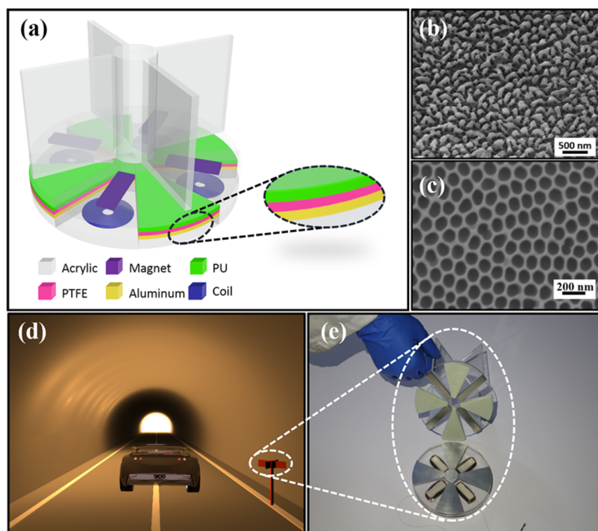
Figure 1. Structural design of self-powered wireless traffic volume system: (a) sketch of the sensor; (b) SEM image of PTFE surface with nanostructure modification; (c) SEM image of aluminum nanopores; (d) schematic diagram of the sensor which is working in the tunnel; (e) enlarged view of the self-power sensing system.
