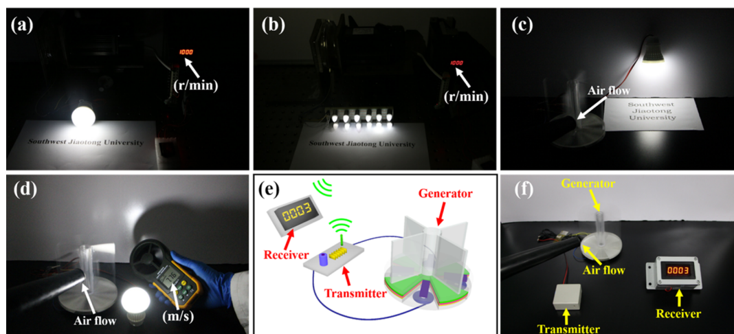
Figure 5. Demonstration of the hybridized nanogenerator as practical power sources and for a self-powered wireless traffic volume sensing system. (a, b) Photographs of a G16 globe light (a) and 12 G4 spot lights (b) that are directly powered by the hybridized nanogenerator in complete darkness (rotation rate: 1000 rpm). (c, d) A G16 globe light was powered for reading illumination in complete darkness by harvesting energy from fresh breeze at a flow speed of 7.76 m/s. (e, f) Schematic diagram (e) and photograph (f) of the wireless traffic volume sensing system that powered by the hybridized nanogenerator.
