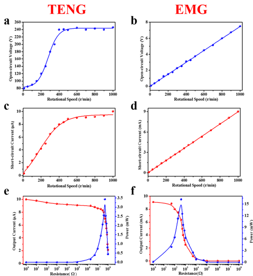
Figure 3. Electrical output performance of the TENG part and EMG part of the hybridized nanogenerator. (a, b) Dependence of the open-circuit voltage of TENG (a) and EMG (b) on rotating speeds ranging from 10 to 1000 rpm. (c, d) Short-circuit current of TENG (c) and EMG (d) with variable rotating speeds ranging from 10 to 1000 rpm. (e, f) Dependence of the output current and power of TENG (e) and EMG (f) on the external resistances.
