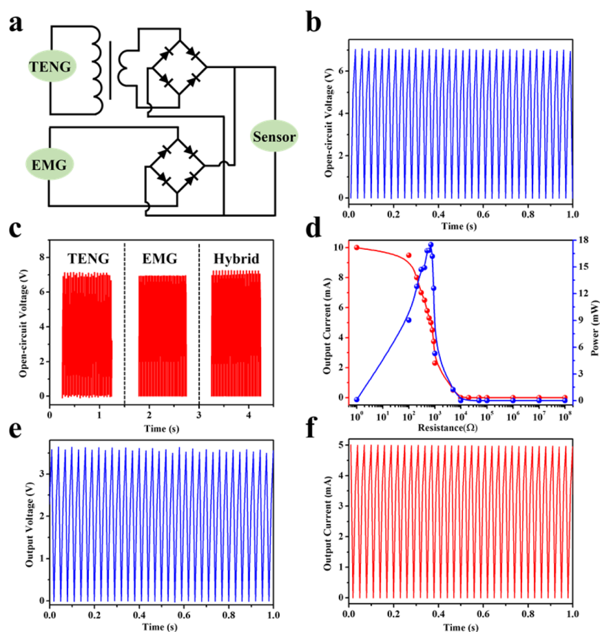
Figure 4. Schematic diagram and electrical output performance of the hybridized nanogenerator: (a) schematic diagram of the self-powered sensing system; (b) open-circuit voltage of TENG with transformer; (c) comparison of open-circuit voltage of TENG with transformer and rectification bridge, EMG with rectification bridge, and the hybridized nanogenerator; (d) dependence of the output current and power of the hybridized device on the external resistances; (e, f) output voltage (e) and current (f) of the hybridized nanogenerator at a loading resistance of 700 \Omega .
