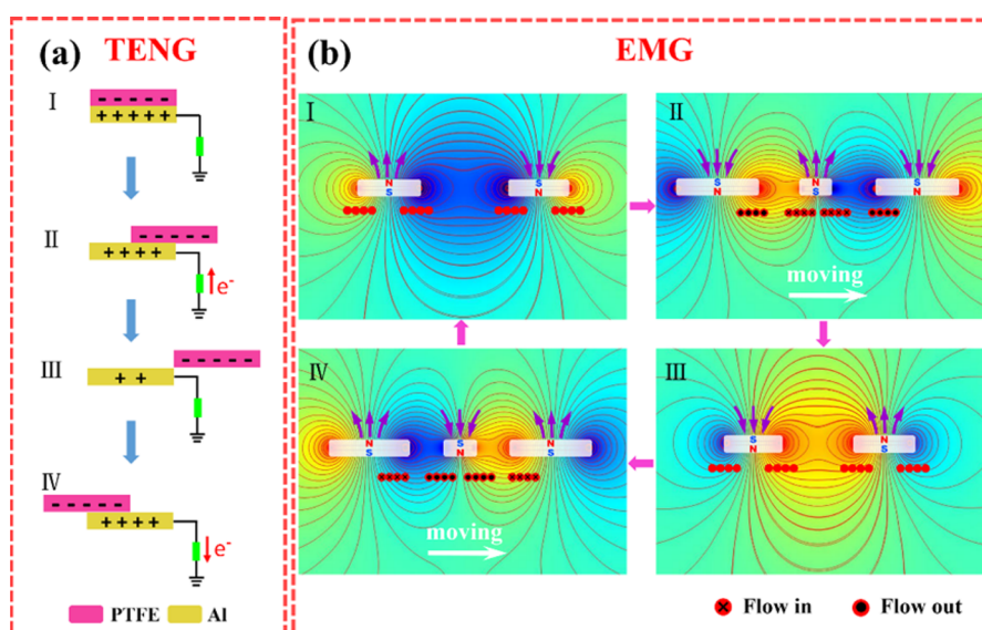
Figure 2. Working principle of the hybridized nanogenerator for power generation: (a) schematic diagram of working principle of TENG. The four process illustrate the charge distribution and electricity generation; (b) schematic diagram of working principle of EMG.
