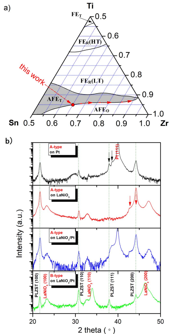
Fig. 1. (a) The phase diagram of the \text{Pb}_{0.097}\text{La}_{0.02}(\text{Zr,Sn,Ti})\text{O}_3 system [25]. (b) XRD patterns of \text{Pb}_{0.97}\text{La}_{0.02}(\text{Zr}_{0.65}\text{Sn}_{0.3}\text{Ti}_{0.05})\text{O}_3 (PLZST) thin films with A-type and B-type annealing modes on Pt, \text{LaNiO}_3 and \text{LaNiO}_3/\text{Pt} bottom electrodes. FE: ferroelectric, AFE: antiferroelectric, T: tetragonal, O: orthorhombic, R: rhombohedral, HT: high temperature, LT: low temperature.
