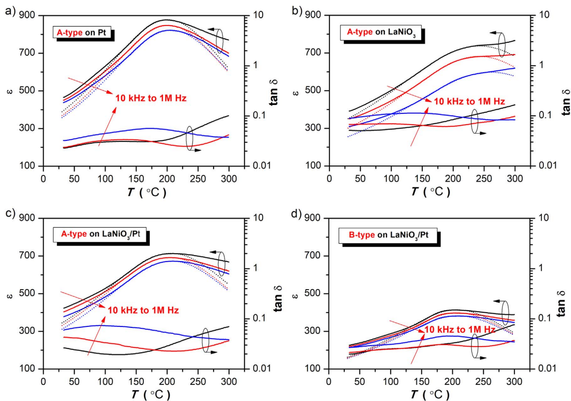
Fig. 4. \epsilon(T) and \tan \delta(T) of PLZST thin films: (a) A-type on Pt electrode, (b) A-type on LaNiO 3 electrode, (c) A-type on LaNiO 3 /Pt composite electrode, and (d) B-type on LaNiO 3 /Pt composite electrode.
