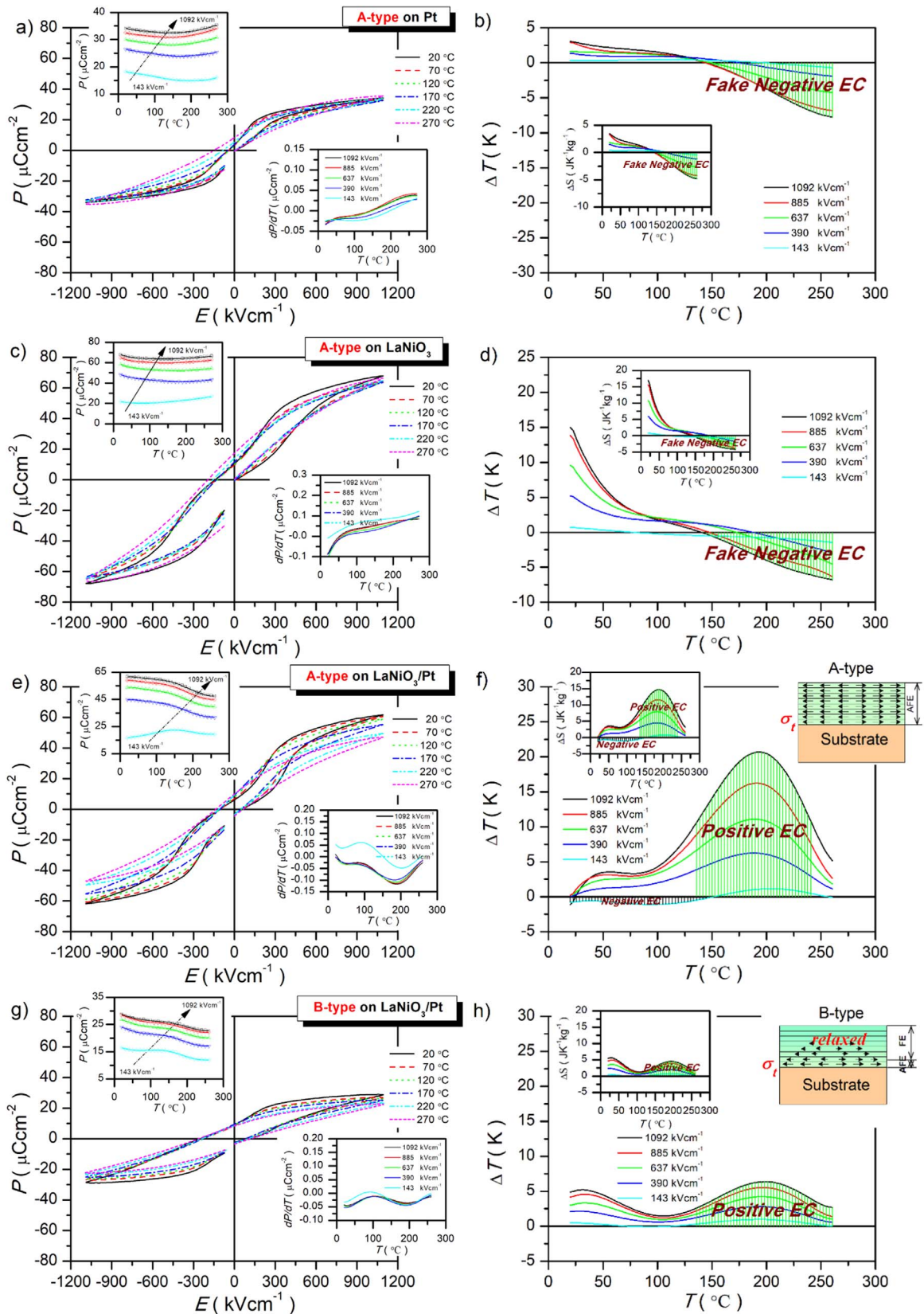
Fig. 5. P - E loops and the corresponding \Delta T(T) of the PLZST thin films at selected temperatures. (a), (b) A-type on Pt electrode. (c), (d) A-type on \text{LaNiO}_3 electrode. (e), (f) A-type on \text{LaNiO}_3/\text{Pt} composite electrode. (g), (h) B-type on \text{LaNiO}_3/\text{Pt} composite electrode. Insets in (a), (c), (e) and (g): P(T) (left upper corner) and dP/dT (right lower corner) at selected electric fields. Insets in (b), (d), and the left upper corners of (f) and (h): \Delta S(T) . Insets in the right upper corners of (f) and (h): schematic diagrams of showing the in-plane thermally induced tensile stress ( \sigma_x ) in thin films.
