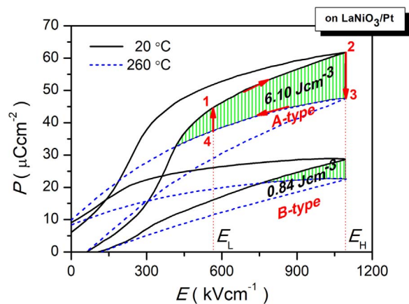
Fig. 6. Olsen cycle diagram of pyroelectric energy harvesting of the PLZST thin film on LaNiO_3/Pt composite electrode.
