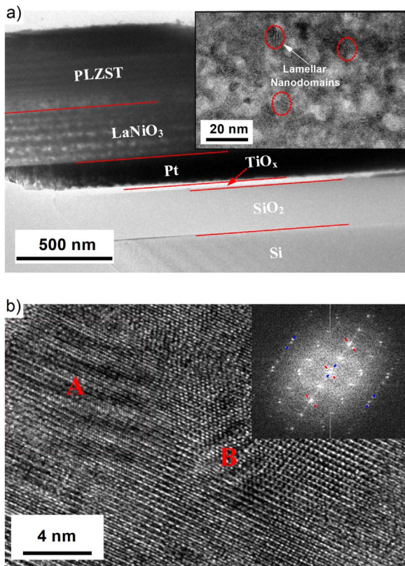
Fig. 3. (a) Cross-sectional TEM image of the PLZST thin film with A-type annealing mode on LaNiO 3 /Pt composite bottom electrode. Inset: magnified part of the thin film. (b) Cross-sectional HRTEM image of two adjacent laminar domains. Inset: the corresponding Fourier transform pattern. The blue or red dots in pairs: superlattice reflections.
