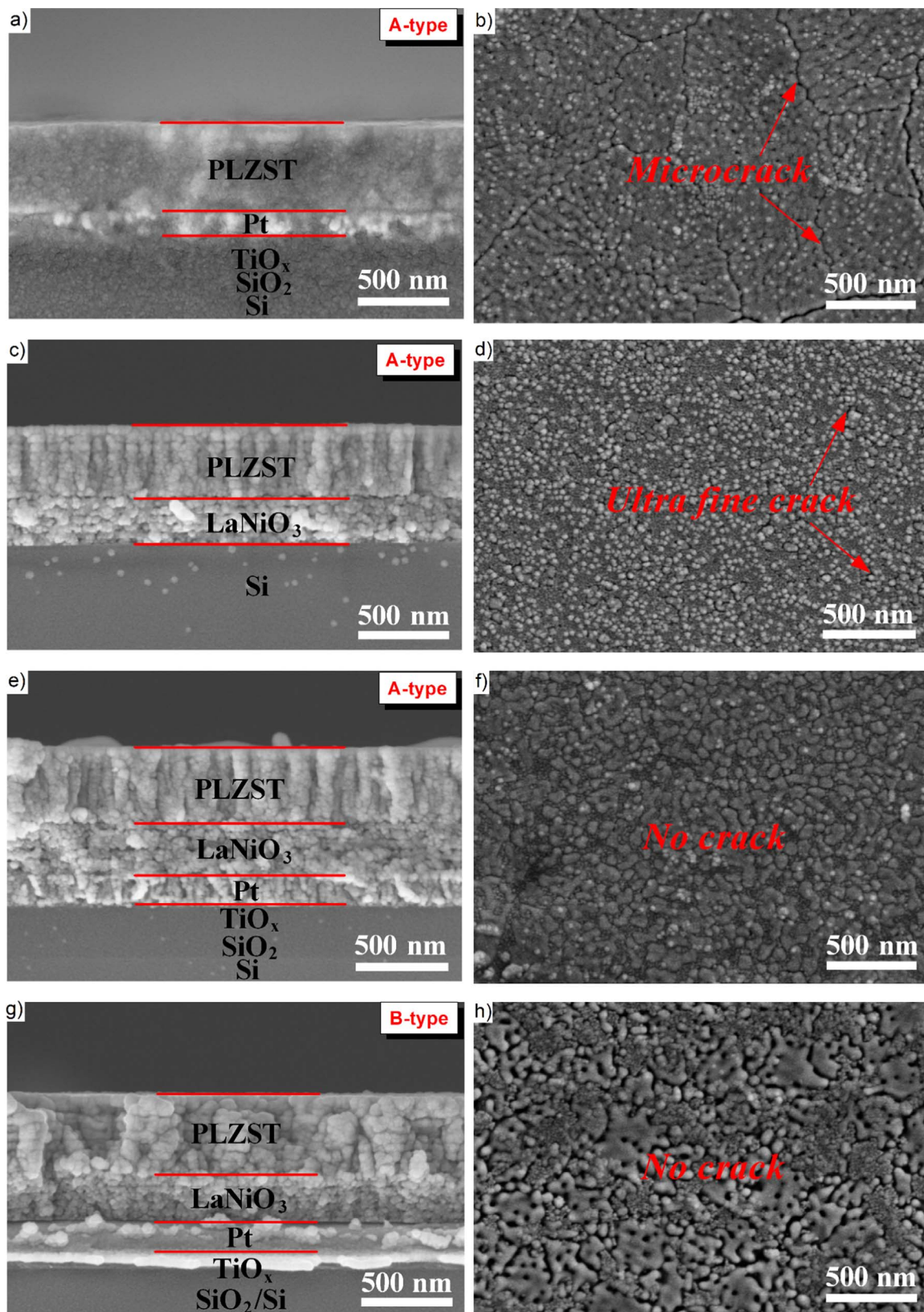
Fig. 2. Cross-sectional and the corresponding surface SEM images of PLZST thin films. (a), (b) A-type on Pt electrode. (c), (d) A-type on LaNiO 3 electrode. (e), (f) A-type on LaNiO 3 /Pt composite electrode. (g), (h) B-type on LaNiO 3 /Pt composite electrode.
