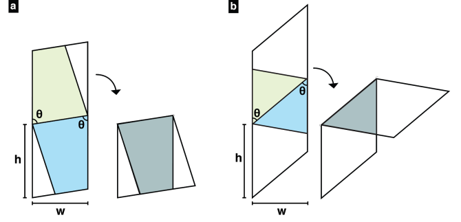
Figure 9. Each Miura folding pattern unit's overlapping part shape changes depending on the unit corner's angle: (a) trapezoid contact area, and (b) triangle contact area.
