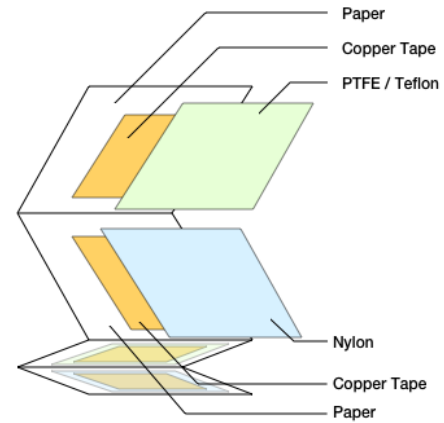
Figure 2. SPIN design: one unit of the energy harvesting structure is formed with a pair of two composite faces. Each side is attached to a paper crease.
