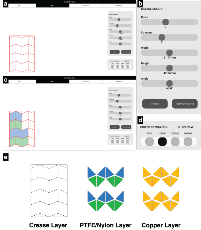
Figure 8. SPIN design editor walkthrough: (a) Select a folding type and adjust parameters; (b) Crease Design palette to adjust parameters (from the top: Rows, Columns, Width, Height, Angle and two buttons for “Reset” and “Export Files”); (c) Select where to apply the self-power modules; (d) Estimate generated power by selecting a resistor; (e) Export files for paper, copper, and PTFE layers of the final design.
