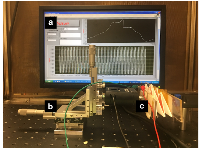
Figure 6. Measurement test setting: (a) computer running software that recording readings; (b) a commercial linear motor that compresses two ends with a specified force, replicating a consistent, repeating fold; (c) a TENG-applied paper crease that we were measuring, in this case the Waterbomb fold.
