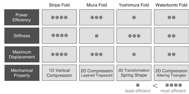
Figure 4. Form module overview.
