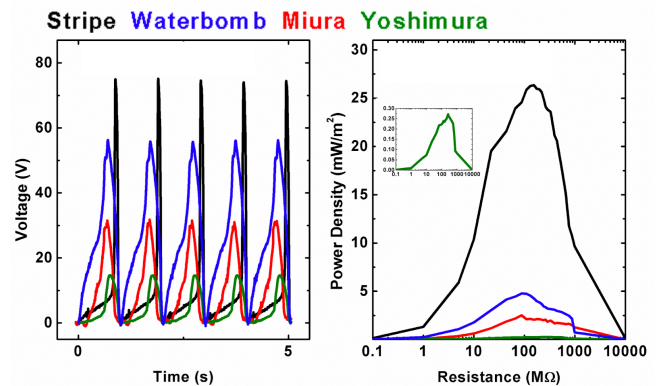
Figure 7. (Left) Open-circuit voltage comparison; (right) power comparison across a period of 15 minutes.
