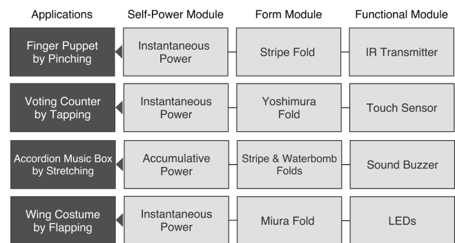
Figure 11. Application overview: we developed four prototypes based on different configurations of three building blocks: power, form and function modules.
