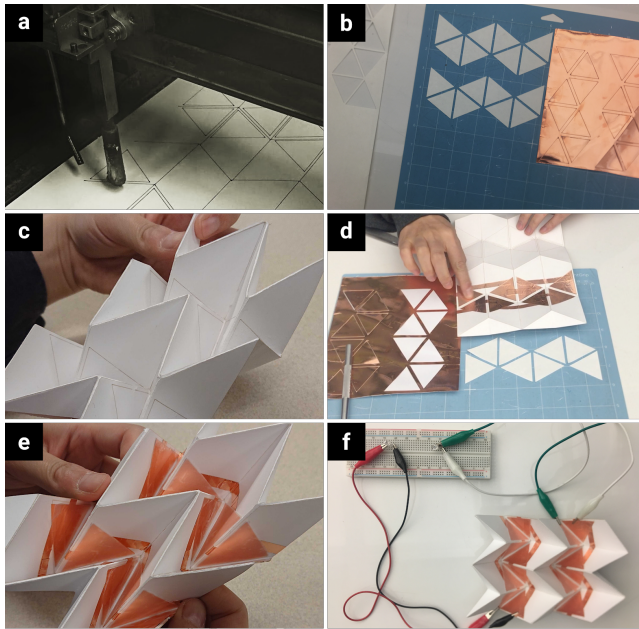
Figure 10. SPIN fabrication step-by-step workflow.
