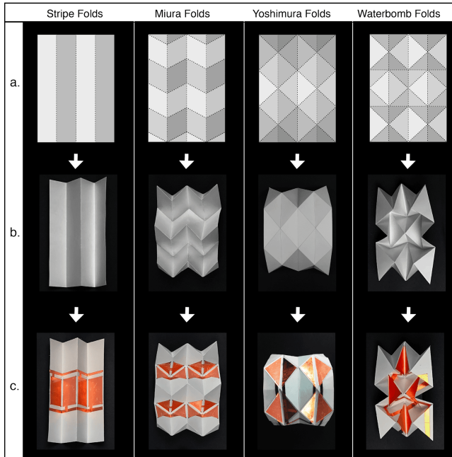
Figure 5. We applied and tested four different crease patterns of the form module and their impacts to the power module efficiency: (a) folding net (b) folded model (c) TENG application.
