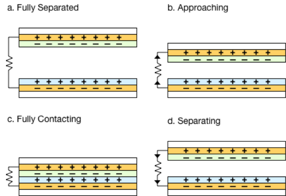
Figure 3. Compressing and expanding layers repeatedly generates triboelectric charges, which can be used to operate connected sensors and actuators.
