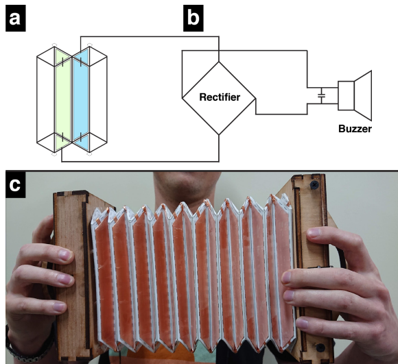
Figure 15. (a) a combined form of a Stripe and Waterbomb folds connected to a melody generator circuit; (b) embedded schematic; (c) as the accordion-looking device is compressed and expanded, it charges electricity and plays a melody.
