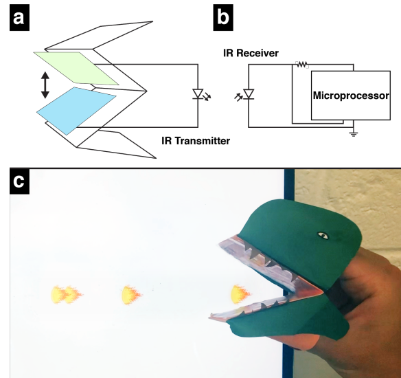
Figure 13. (a) connecting an IR transmitter with a Stripe fold; (b) embedded schematic; (c) as the dinosaur puppet opens and closes its mouth, the screen behind connected to the IR receiver generates shooting fire graphics.
